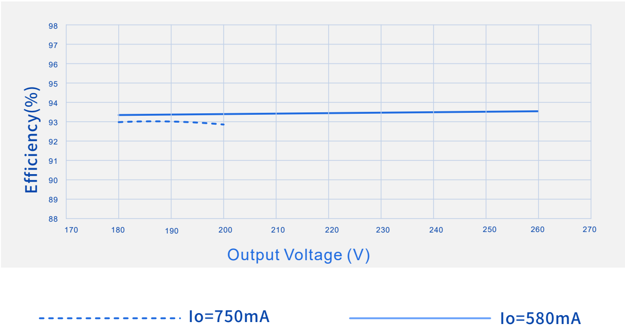
Efficiency Vs. Output Voltage (Vin=198Vac)
